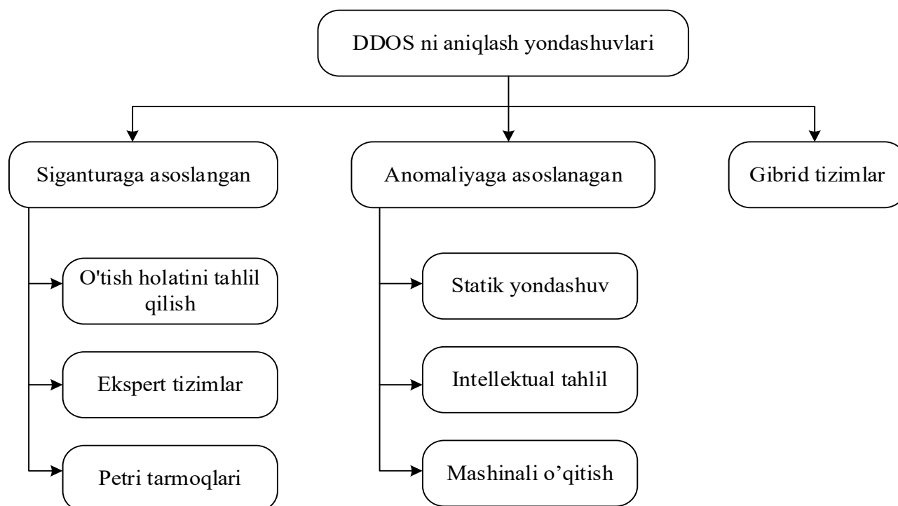
1-rasm. DDOS hujumni aniqlash yondashuvlari
