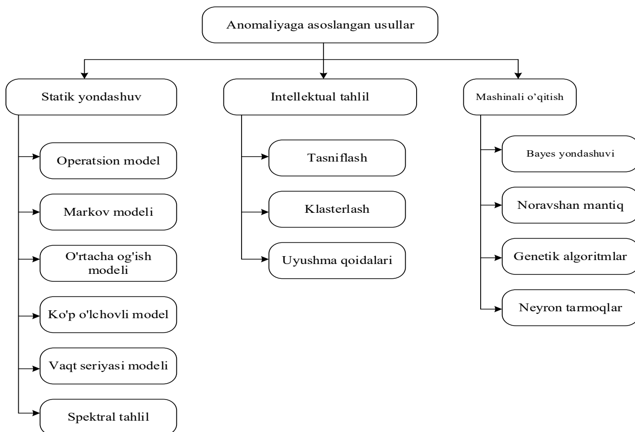
2-rasm. Anomaliyalarga asoslangan usullarning tasnifi
